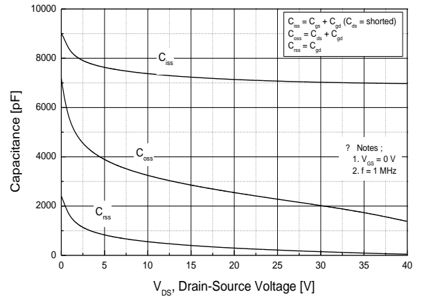
Fig.8 Capacitance Characteristics
