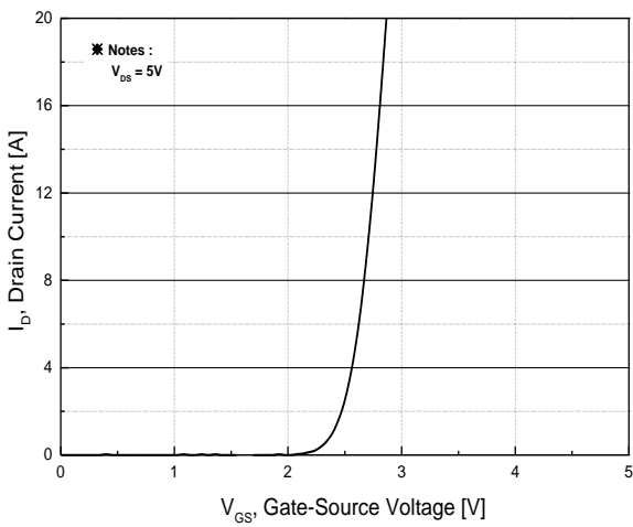
Fig.5 Transfer Characteristics
