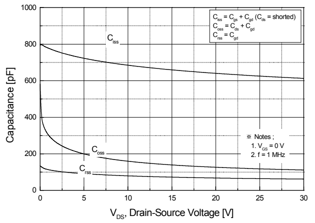
Fig.8 Capacitance Characteristics
