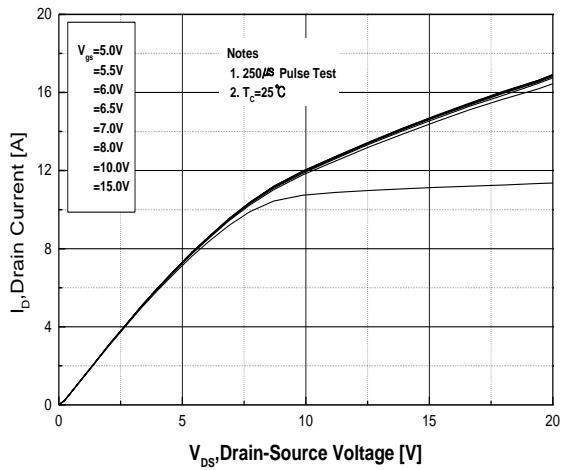
Fig.1 On-Region Characteristics
