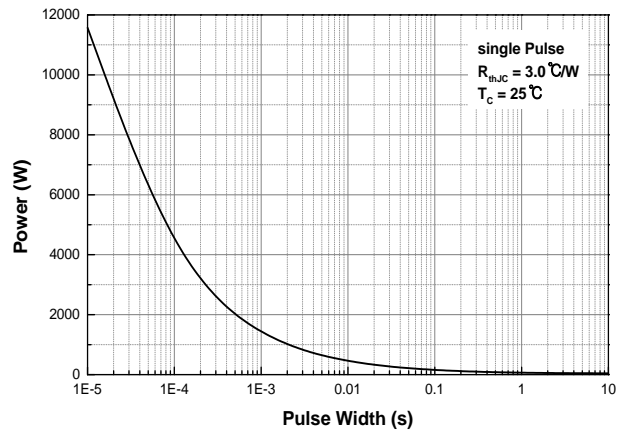
Fig.12 Single Pulse Maximum Power Dissipation
