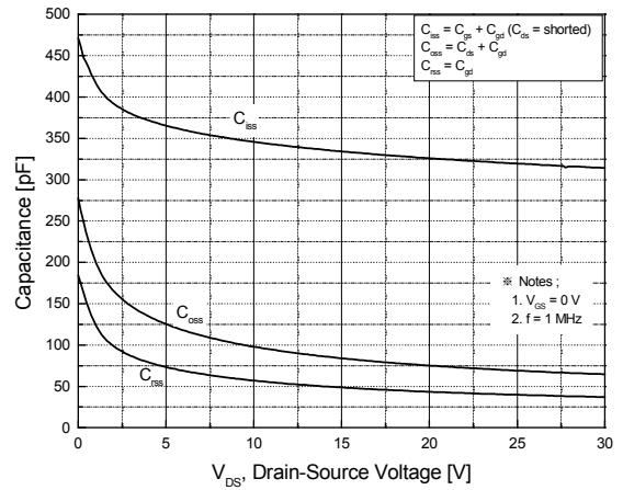
Fig.8 Capacitance Characteristics
