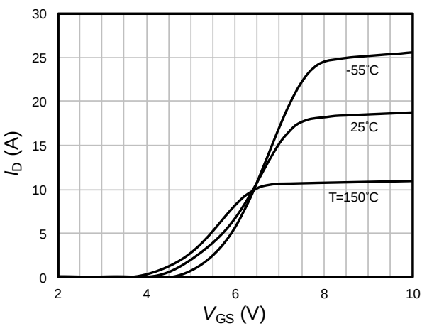
Fig.5 Transfer characteristics
